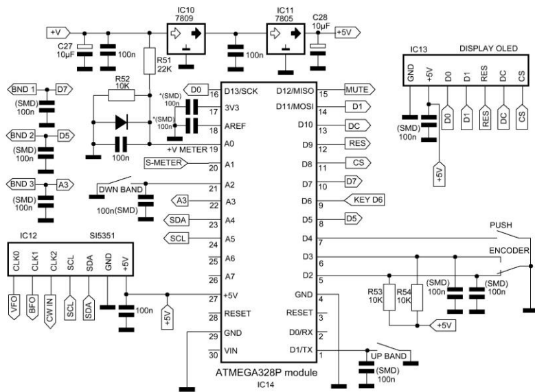
SI5351 EGV-9B v1 All SMD capacitors on PCB bottom layer
